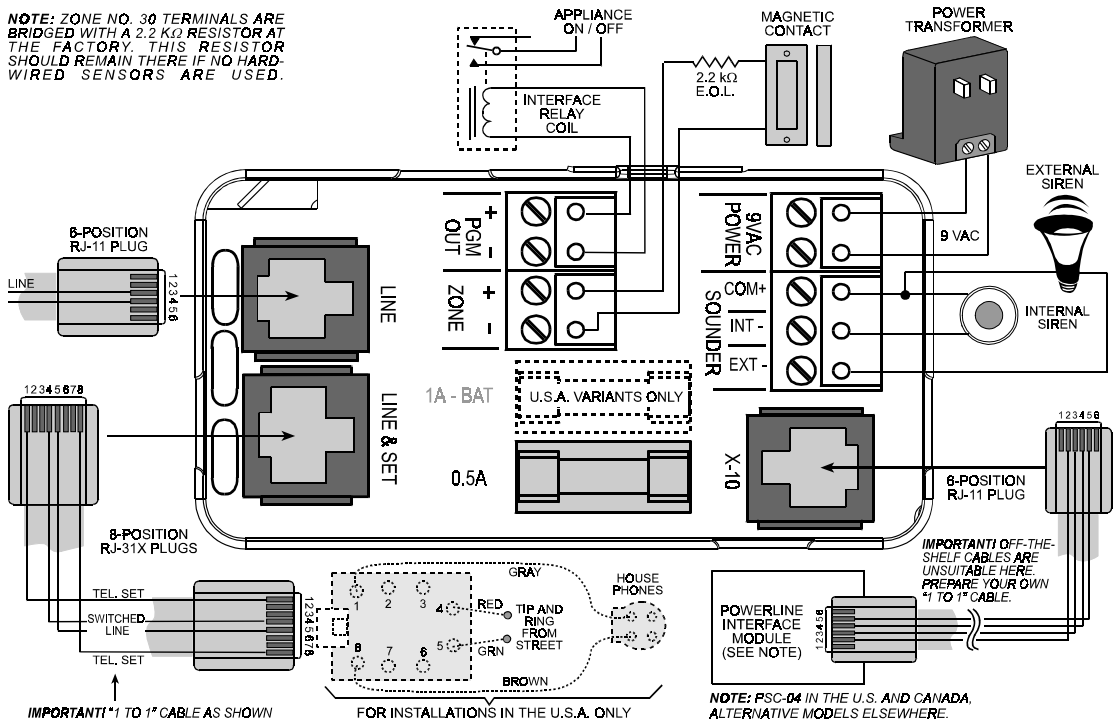
Figure 10. Wiring Diagram
