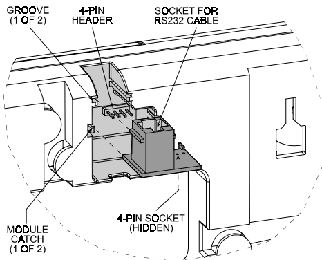
Figure 28. Inserting the RS232 Module
