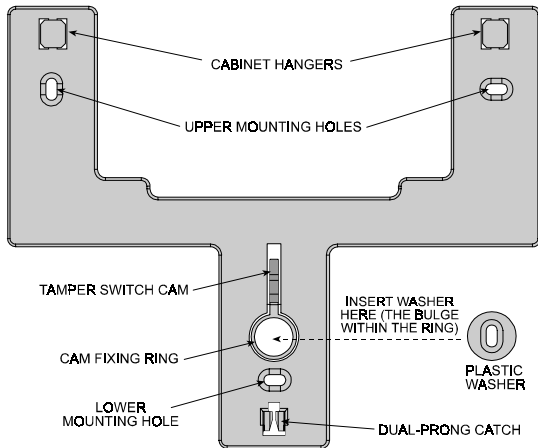
Figure 8. Bracket - Front View
