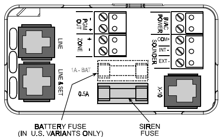
Figure 32. Fuse Locations
